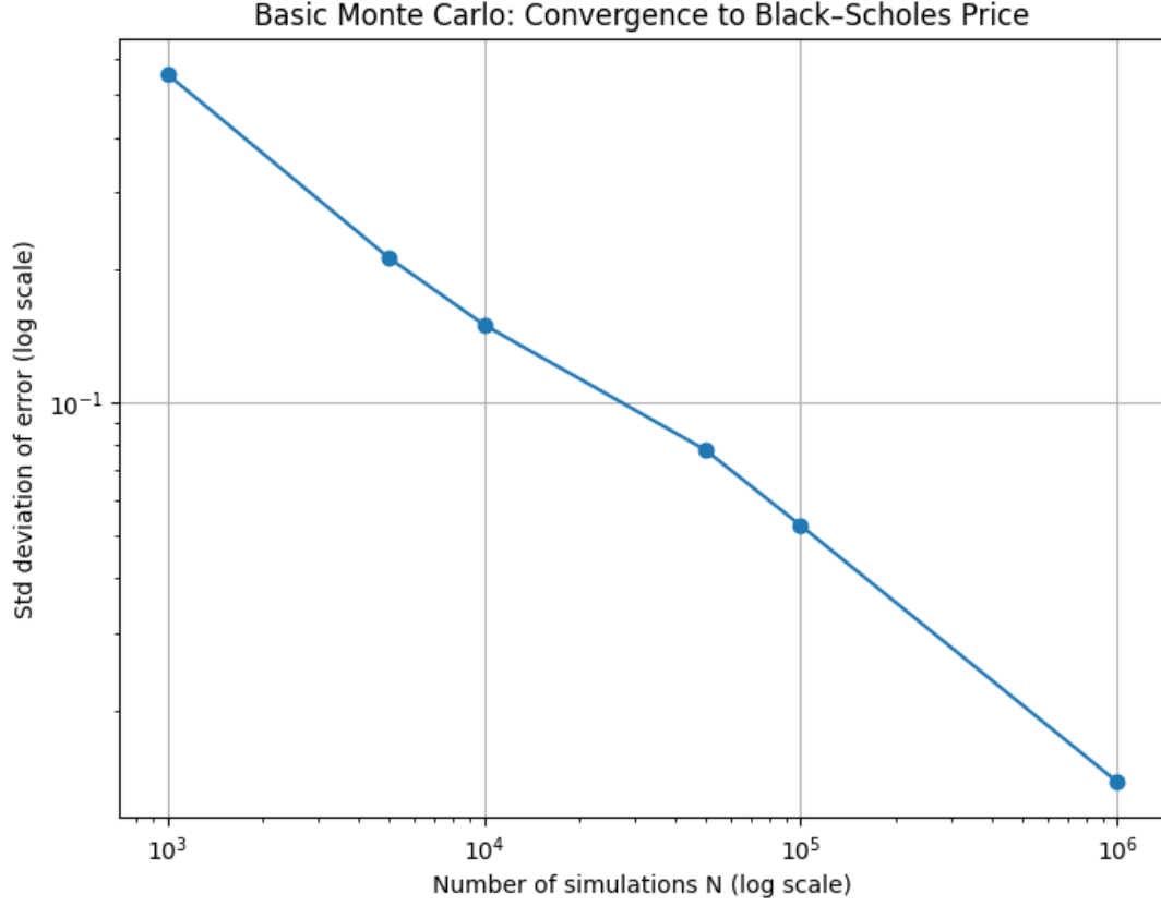
Figure 1: Error convergence of the basic Monte Carlo estimator. The pricing error decreases at the expected rate N^{-1/2} , but the variance remains high for large values of N .
